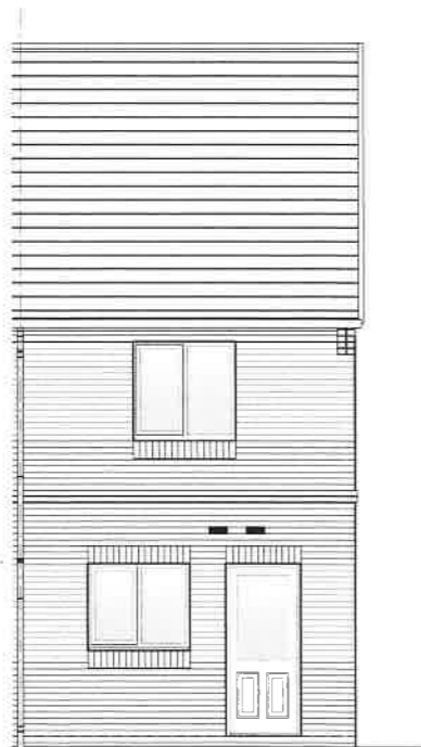
Rear Elevation
